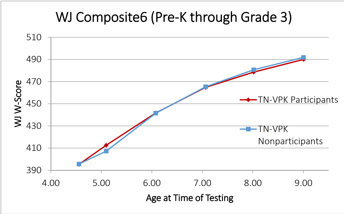
Figure 1: W-Scores on WJ Composite6 for the TN-VPK Participant and Non-Participant Groups on Each Wave of Measurement
